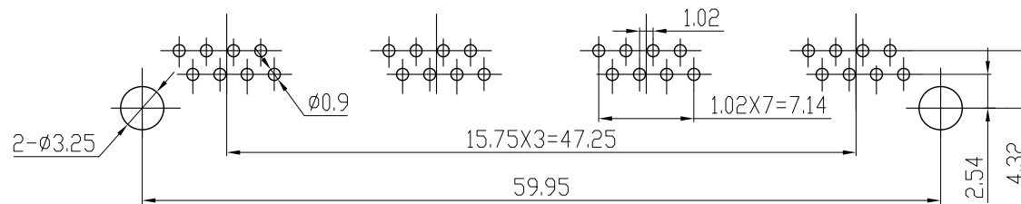
PC Board Layout
